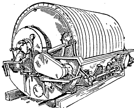
FIG 5 - OLIVER FILTER (AGITATOR SIDE)
